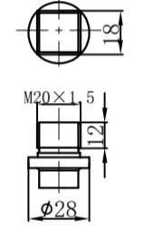
⑬ 放油螺塞 Drain plug
