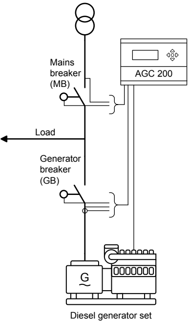
AGC 213 Mains failure, with separate transducer: Peak shaving, load takeover and mains power export
