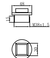
⑬ 放油螺塞 Drain plug
