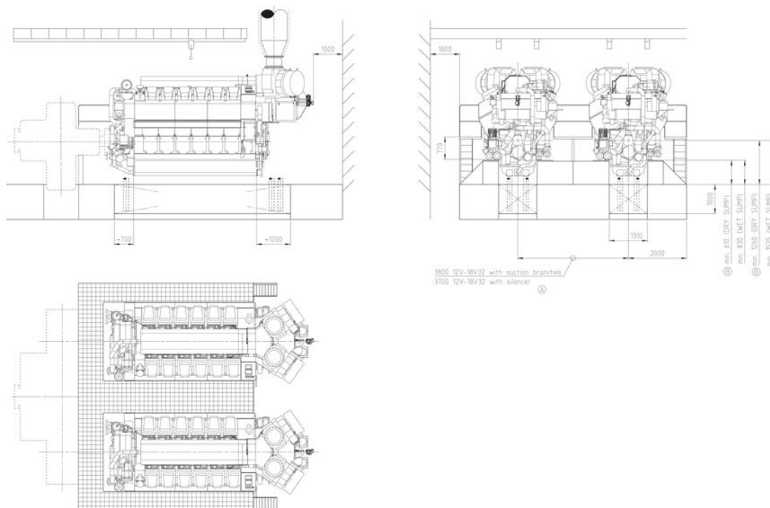
Fig 18-2 V engines, turbocharger in free end (DAAE042488B)
