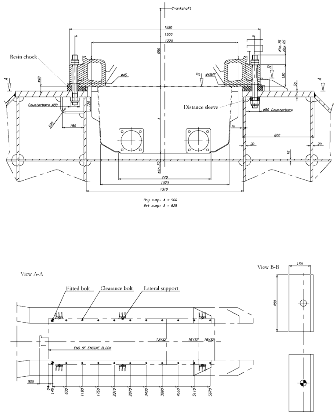
Fig 15-4 Main engine seating and fastening, V engines, resin chocks (1V69A0146g)
