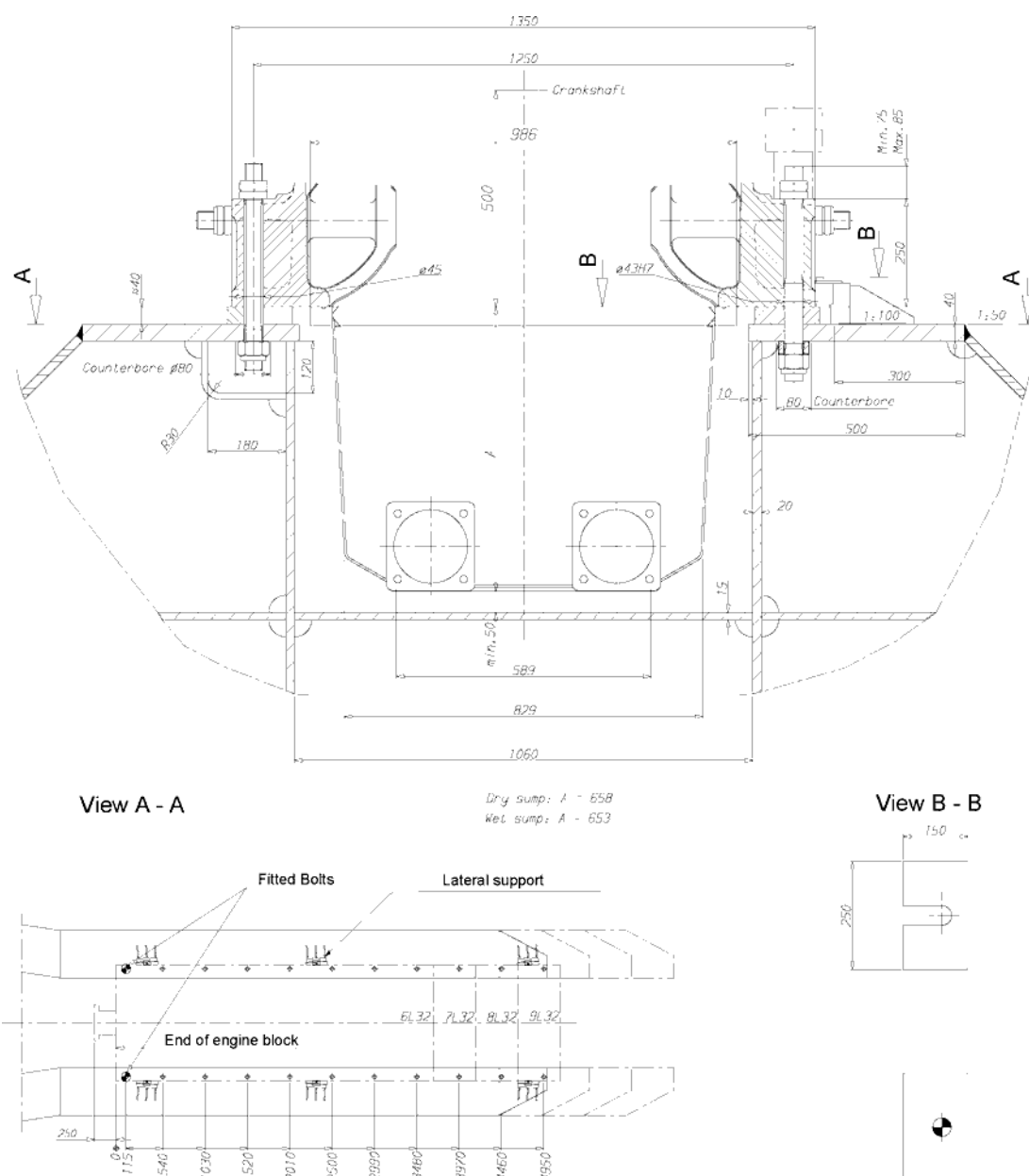
Fig 15-1 Main engine seating and fastening, in-line engines, steel chocks (1V69A0144G)
