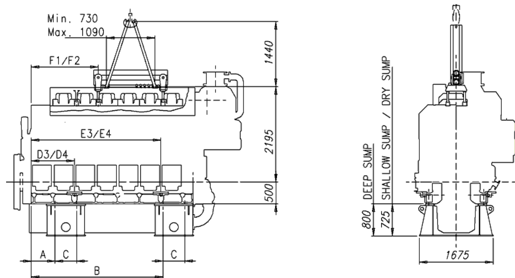
Fig 19-1 Lifting of main engines, in-line engines (2V83D0253F)
