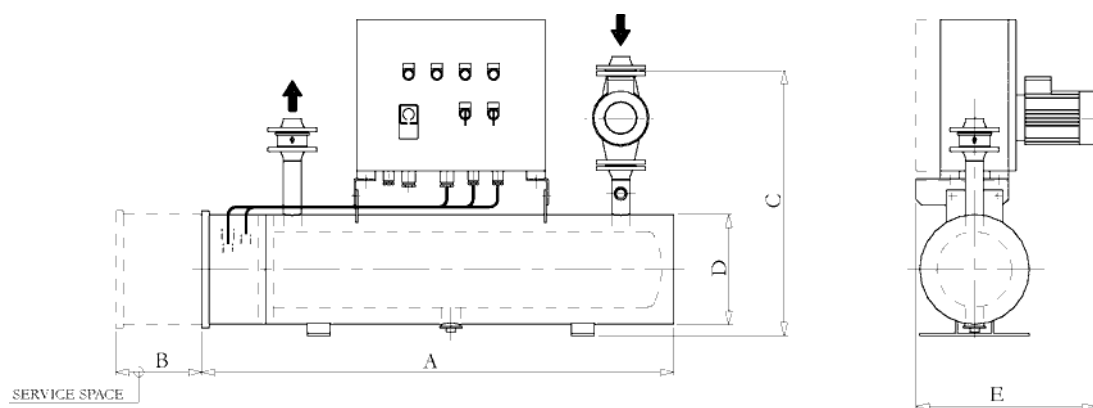
Fig 9-10 Preheating unit, electric (3V60L0562C).
