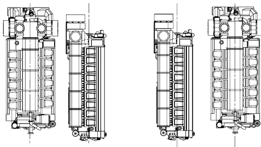
Fig 18-8 Example of father-and-son arrangement, 9L32 + 12V32, TC in flywheel end (DAAE057212)
