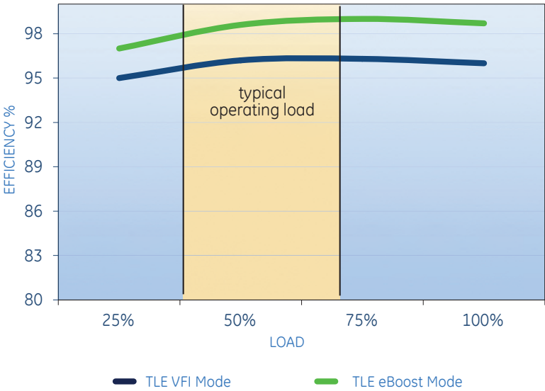
TLE 200 kW UPS EFFICIENCY TLE series delivers efficiency up to 96.5% in double conversion (VFI) mode and 99% in eBoost operating mode
