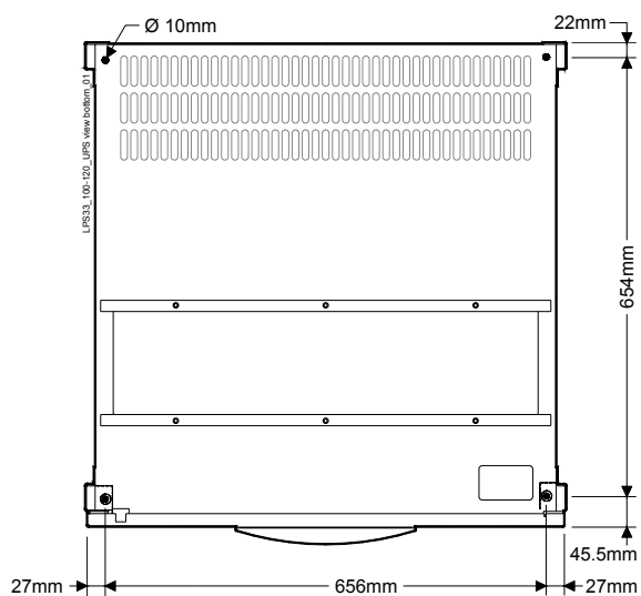
Рис. 4.4-6 LP 33 Series / 100 - 120 кВА - UPS cabinet floor fixing points
