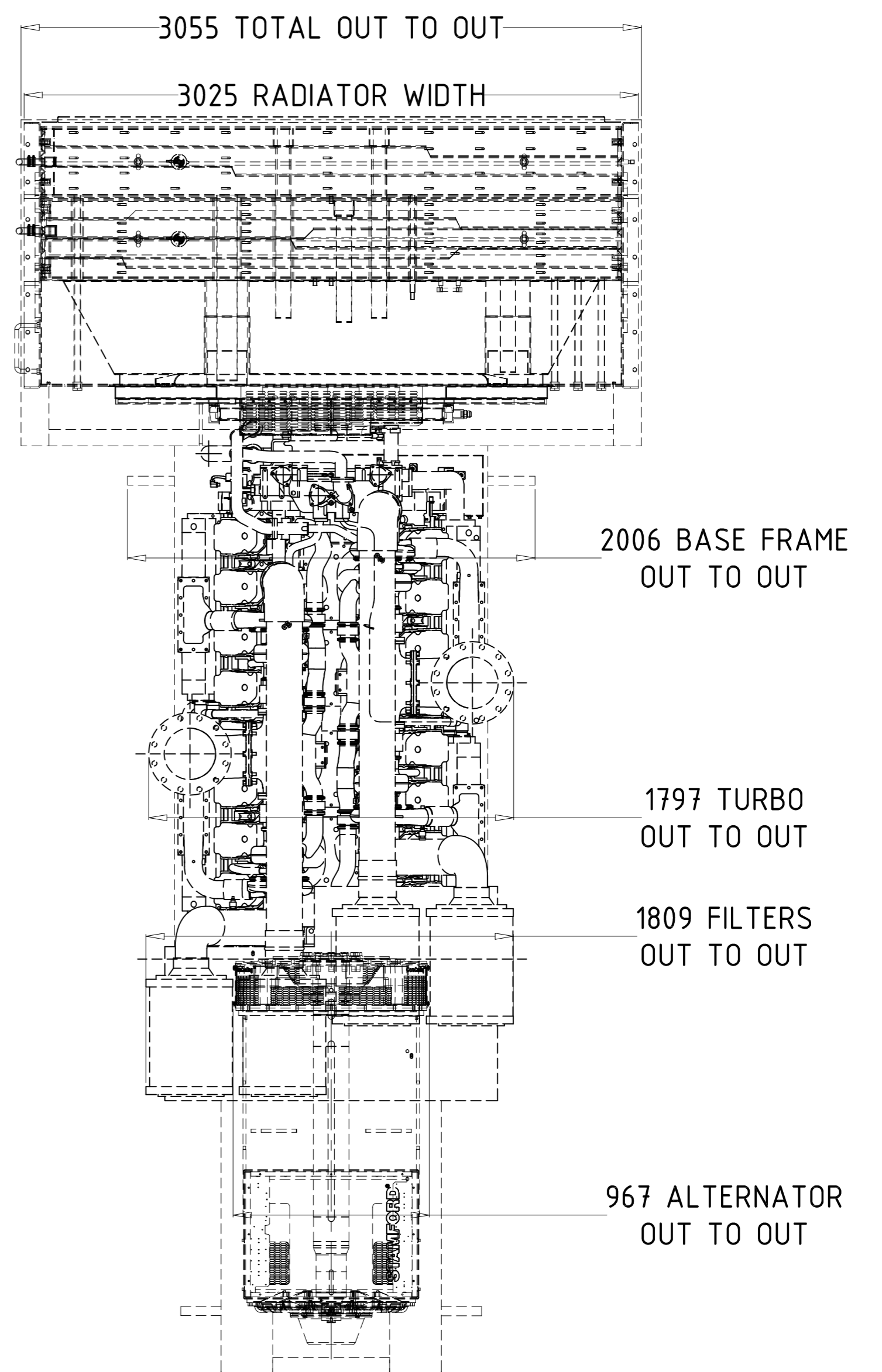
TOP VIEW
